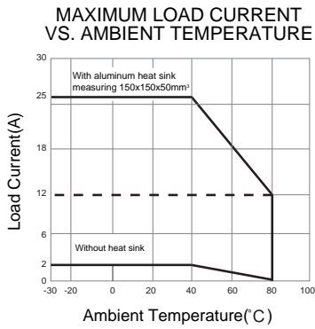
JGX-1505FB/D24Z25&D38Z25
