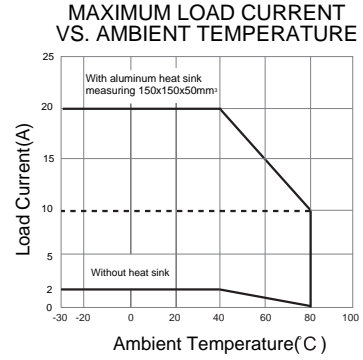
JGX-1505FB/D24Z20&D38Z20
