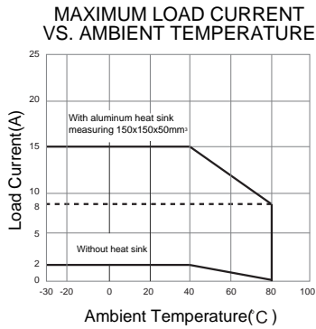
JGX-1505FB/D24Z15&D38Z15
