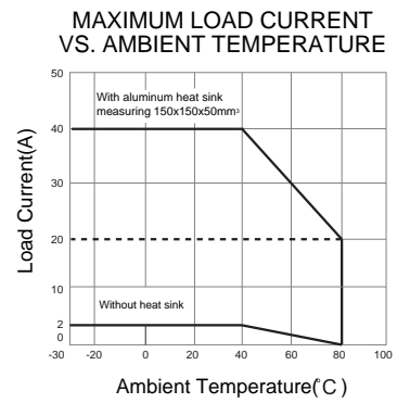
JGX-1505FB/D24Z40&D38Z40
